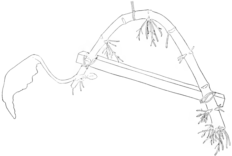
FIG. 67.—Stem bent passively with convexity on upper side. Roots grow on the lower concave side of the stem.
